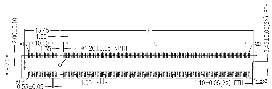
P.C.B. LAYOUT(T=1.60mm) COMPONENT SIDE
