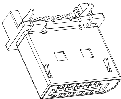
Connector (9WDPC20XL1PU3)
