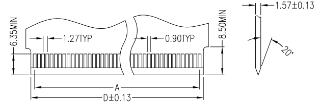
Daughter Card Requirements (±0.05)
